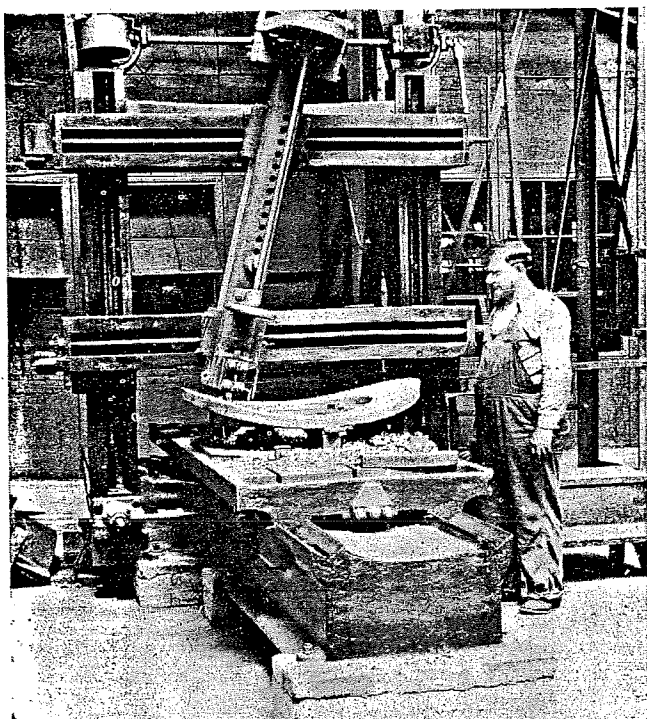
The inner surface of the dome flange being machined in a radius planer
