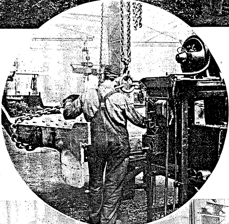
(Left) — Drilling throat sheet rivet holes on a horizontal drill
