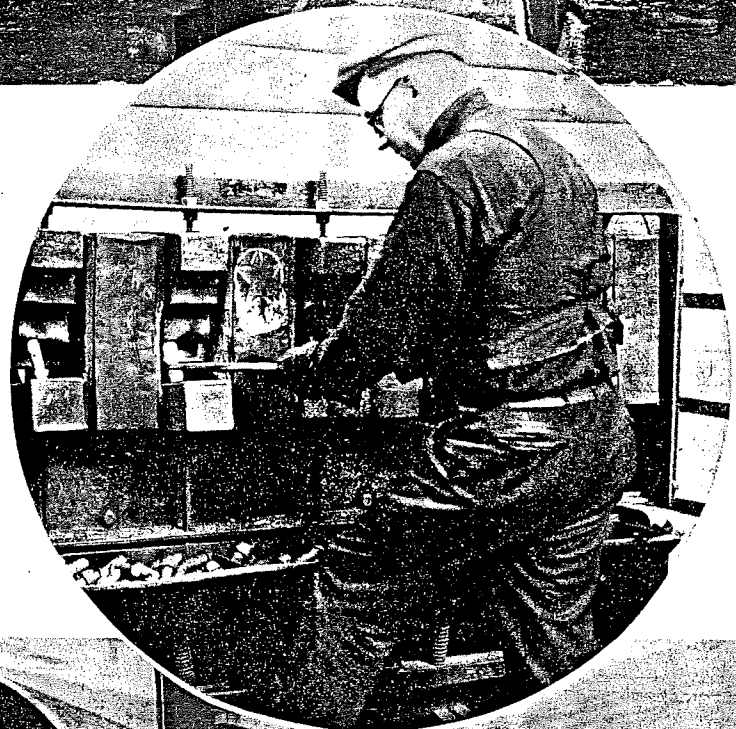
(Right) — Each bull riveter is equipped with a Berwick electric rivet heater
