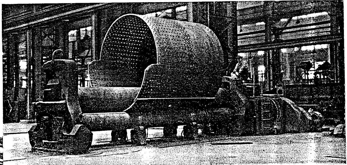
(Right) Final rolling operation on a cylindrical boiler course
