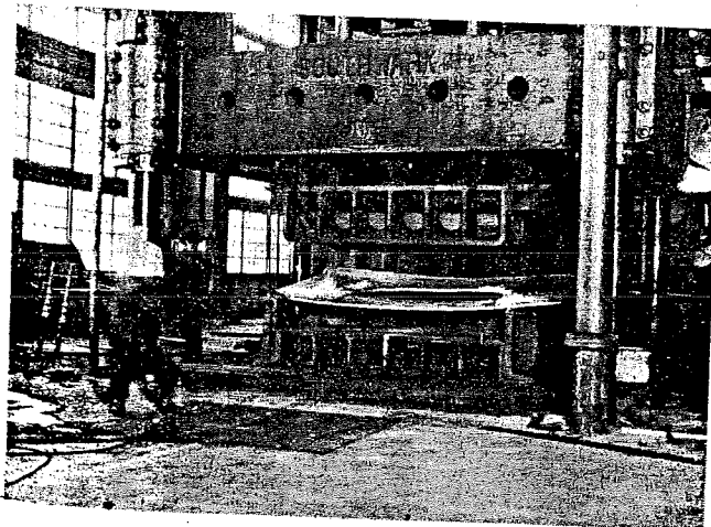
Throat sheet in the 1160-ton Southwark press
