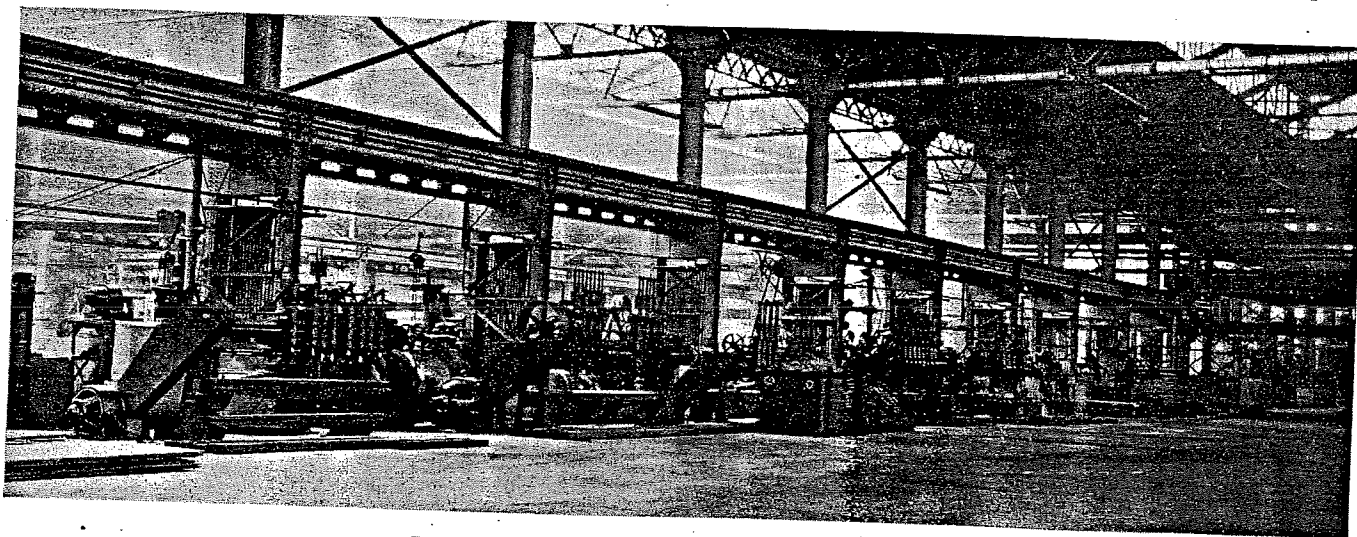
Bay No. 9 showing five 8-spindle drilling machines
