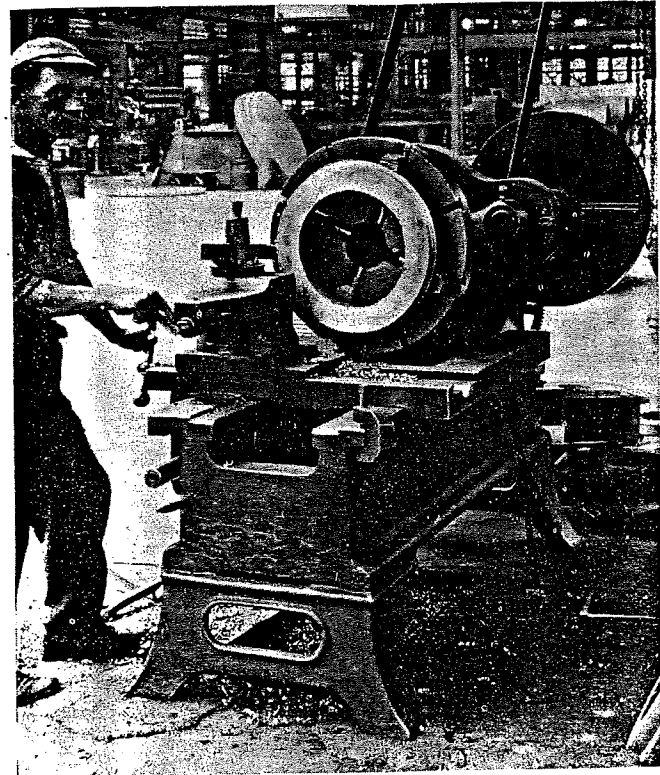
Steam pipe ring set up in a lathe for machining
