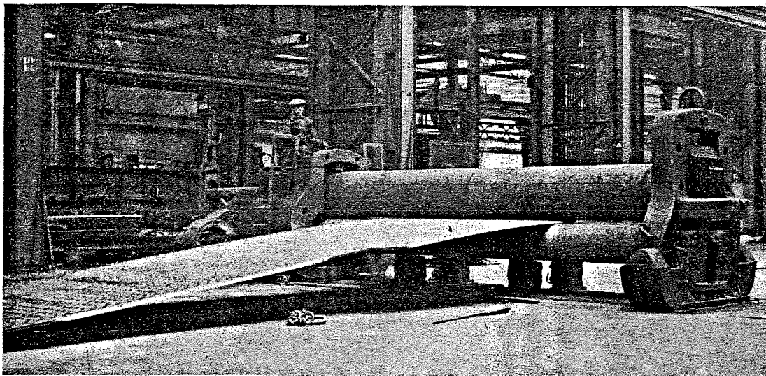
(Above) Partially rolled boiler course
