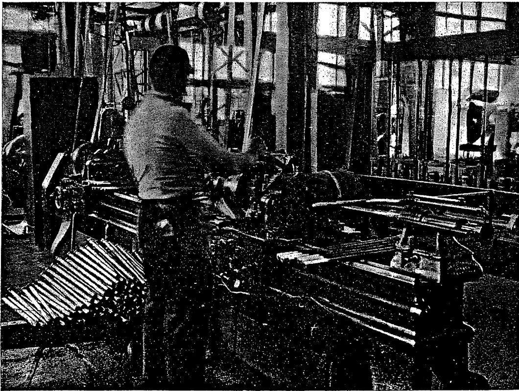
Threading the taper and cutting head grooves in crown staybolts
