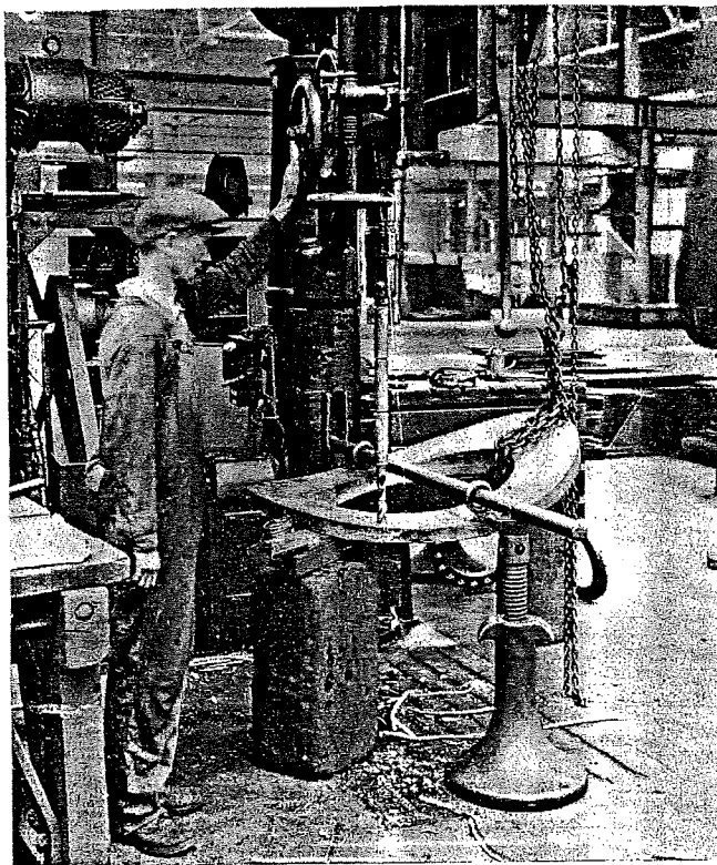
Drilling dome flange rivet holes—note holding jig
