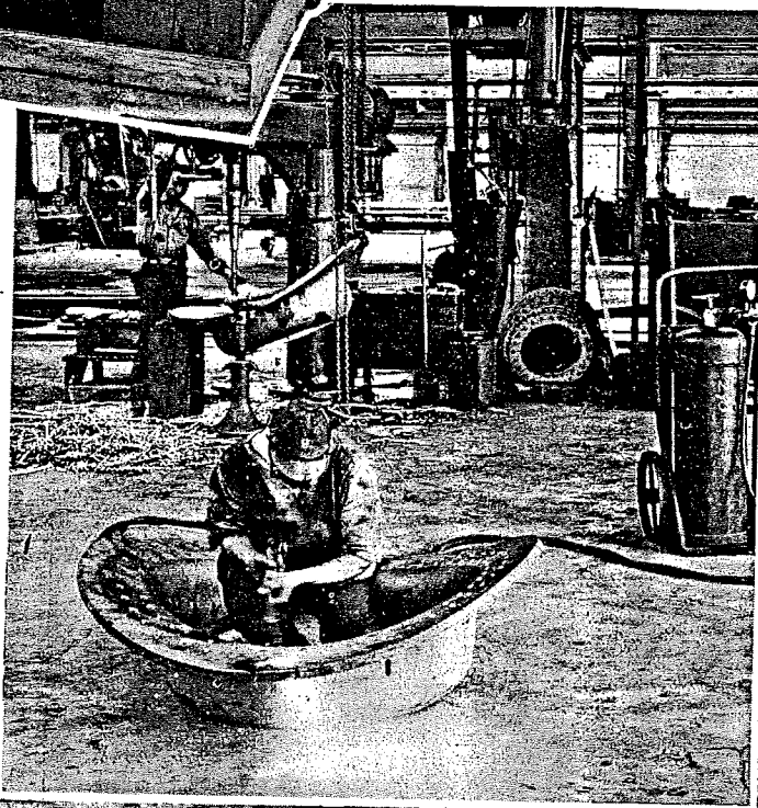
(Above) — Laying out the dome flange holes and edge
