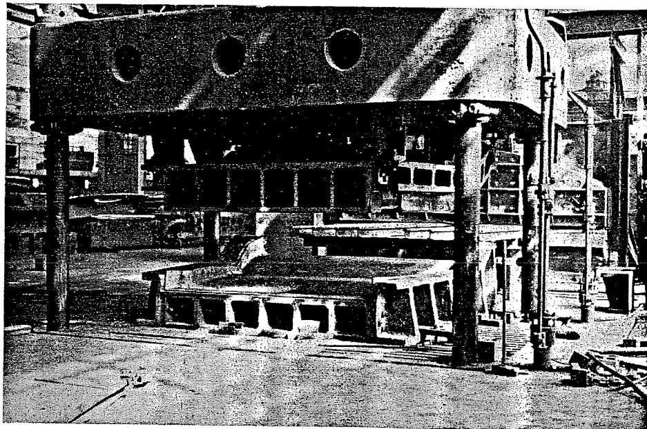
Throat sheet dies set up in an R. D. Wood 4-post hydraulic flanger
