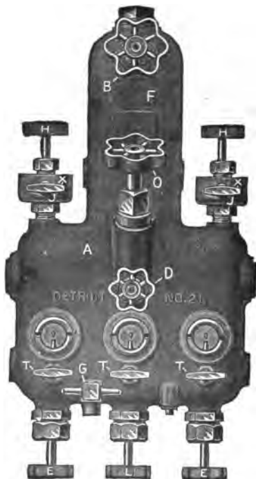
FIG. 51.—DETROIT TRIPPLE-FEED LUBRICATOR.
