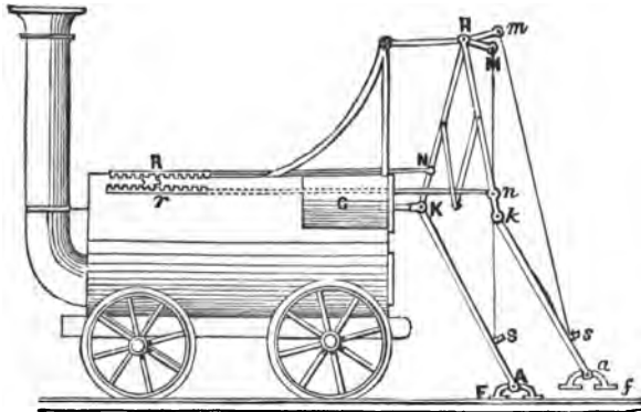
WILLIAM BRUNTON LOCOMOTIVE.
