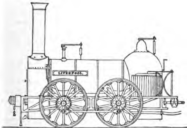
FIG. 17.—BURY'S ORIGINAL "LIVERPOOL," THE FIRST ENGINE WITH INSIDE CYLINDERS AND CRANKED DRIVING AXLE. COUPLED WHEELS, 6ft. DIAMETER.
