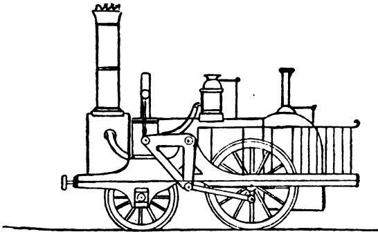
FIG. 24.—ROBERTS'S "EXPERIMENT," WITH VERTICAL CYLINDERS, BELL-CRANK CONNECTING-ROD, AND CYLINDER VALVES
