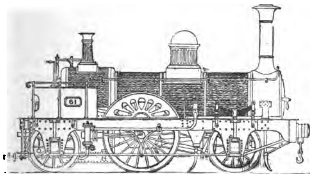
FIG. 43.—"No. 61," LONDON AND BRIGHTON RAILWAY
