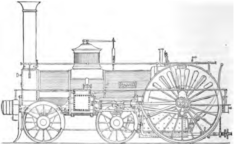
FIG. 40.—THE "NAMUR," THE FIRST ENGINE BUILT ON CRAMPTON'S PRINCIPLE
