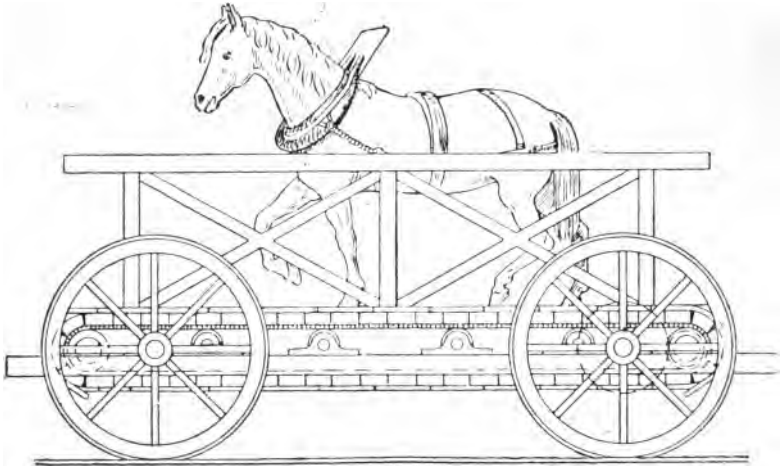
FIG. 16.—WINANS' "CYCLOPED" HORSE LOCOMOTIVE
