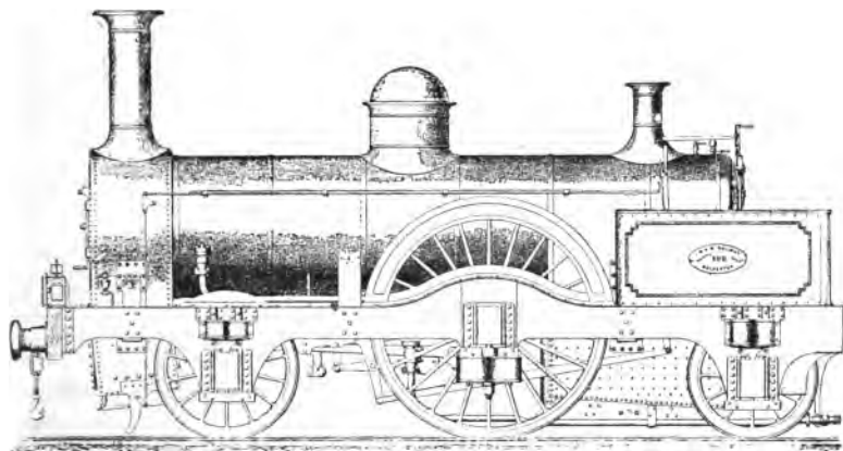
FIG. 64.—McCONNELL'S "300," LONDON AND NORTH WESTERN RAILWAY
