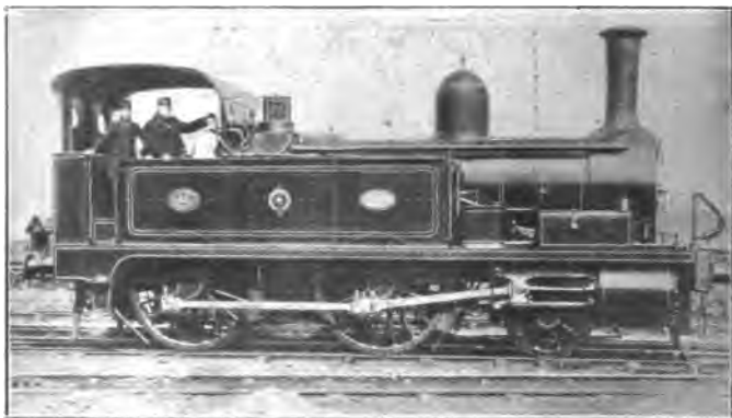
Fig. 144.—4-COUPLED TANK ENGINE WITH OUTSIDE CYLINDERS, NORTH STAFFORDSHIRE RAILWAY.
