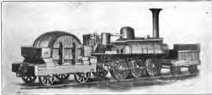
FIG. 22.—"WILBERFORCE," A STOCKTON & DARLINGTON RAILWAY LOCOMOTIVE
