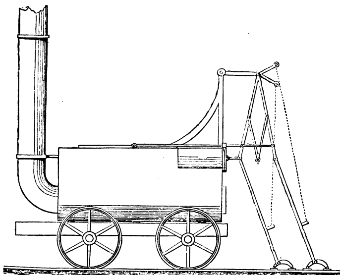
FIG. 3.--BRUNTON'S "MECHANICAL TRAVELLER" LOCOMOTIVE
