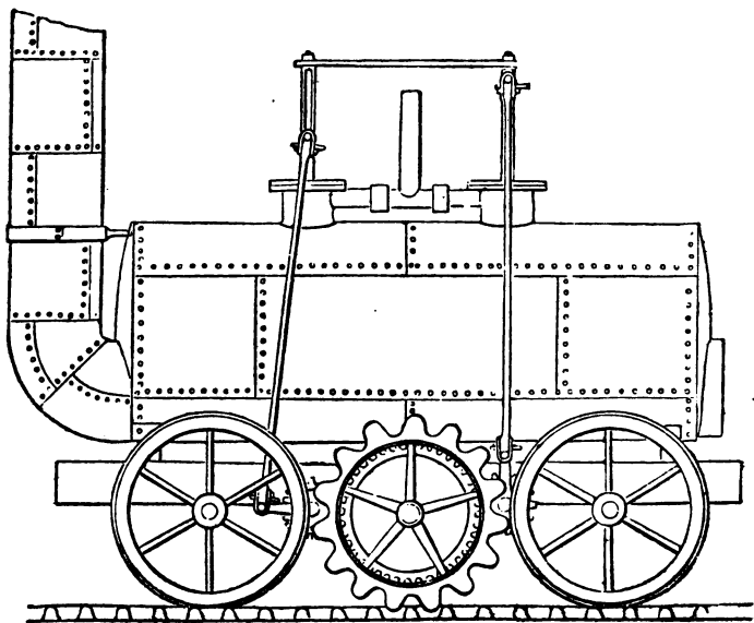
FIG. 2.—LOCOMOTIVE BUILT BY MURRAY FOR BLENKINSOPP'S RAILWAY
