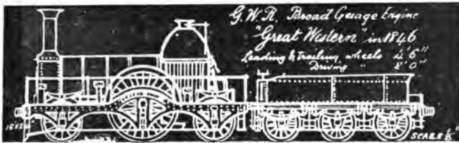
FIG. 38.—THE "GREAT WESTERN" BROAD-GAUGE ENGINE AS ORIGINALLY CONSTRUCTED
