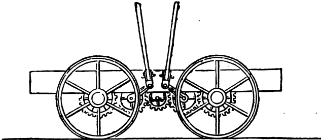
FIG. 6.—STEPHENSON'S INITIAL DRIVING GEAR FOR LOCOMOTIVES
