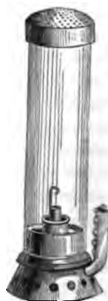
STEPHENSON'S SAFETY LAMP.
