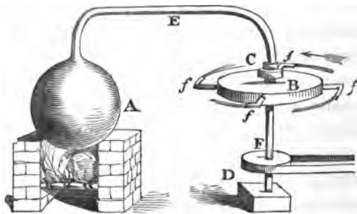
FIG. 1.—HERO'S ENGINE.
