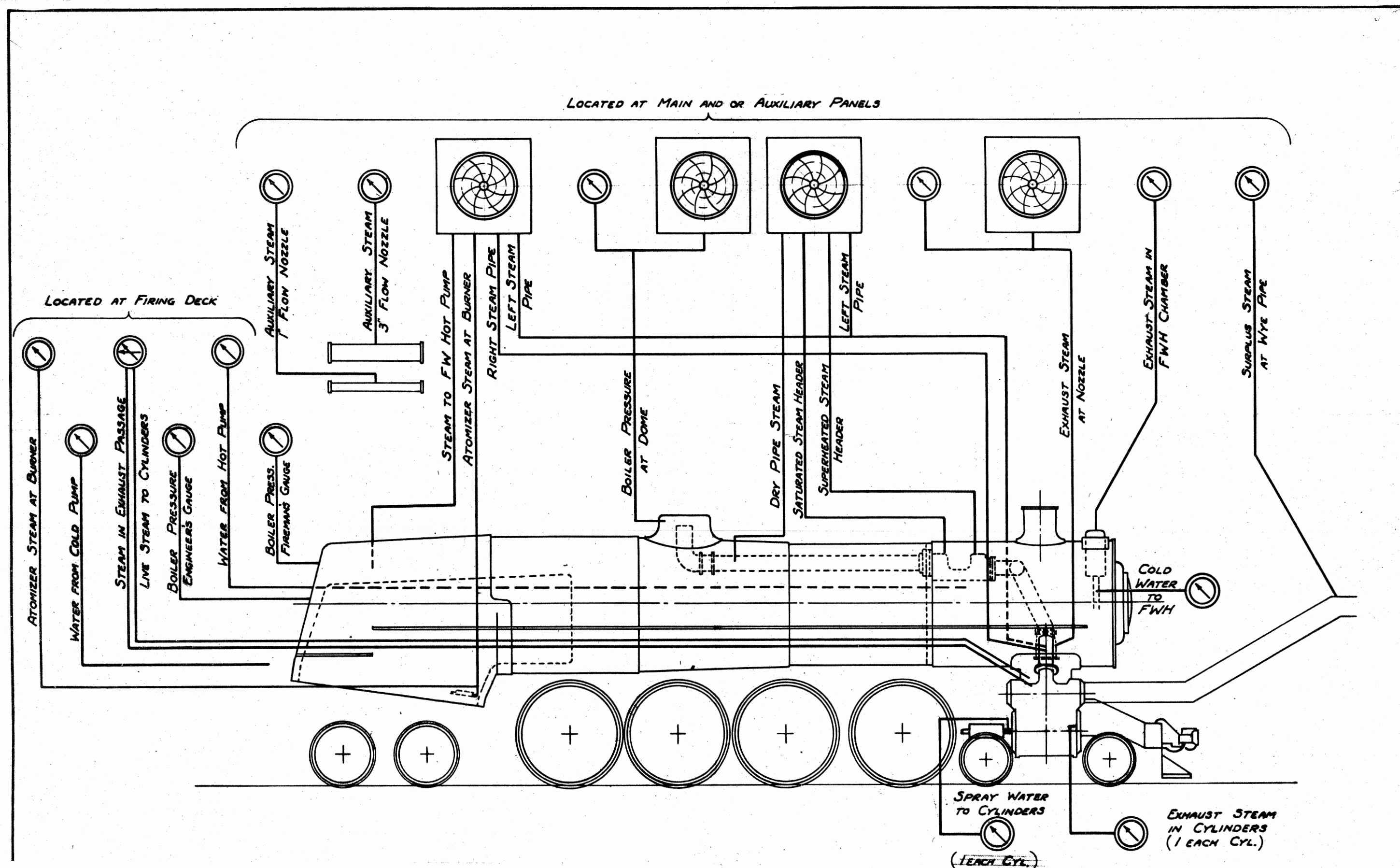
FIG. 8 PRESSURE MEASURING ARRANGEMENT
